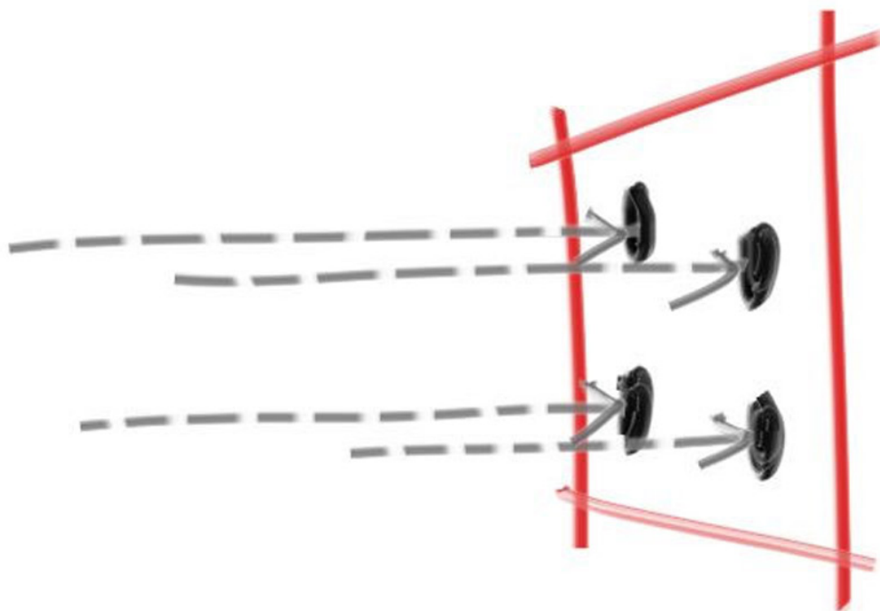
Figure 8: Pixel samples
