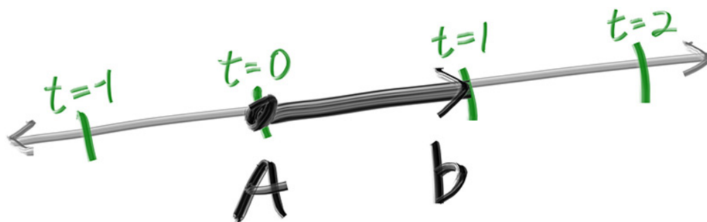
Figure 2: Linear interpolation
