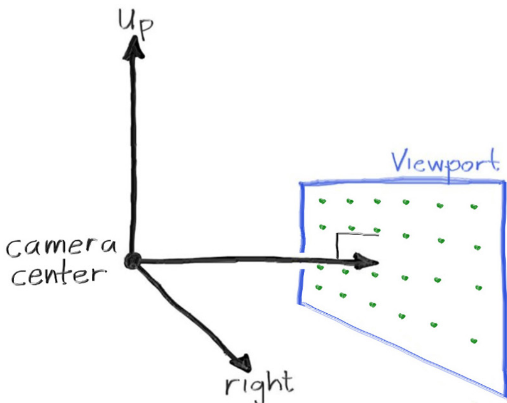
Figure 3: Camera geometry
